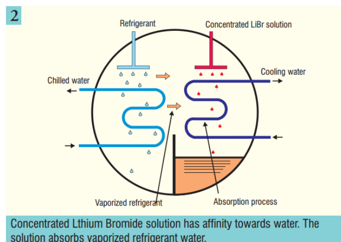
Figure 6. Trane (Thermax) Cooling System – Concentrated LiBr
