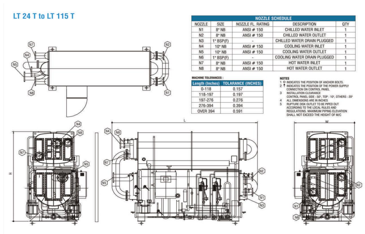
Figure 11. Dimensions of the Absorption Chiller
