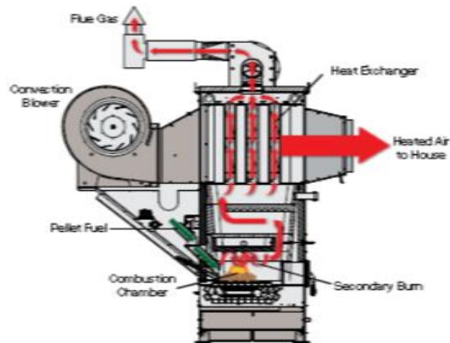
Figure 3. Biomass Furnace Diagram
