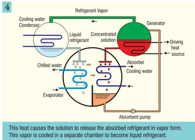
Figure 8. Trane (Thermax) Cooling System – Liquid Refrigerant
