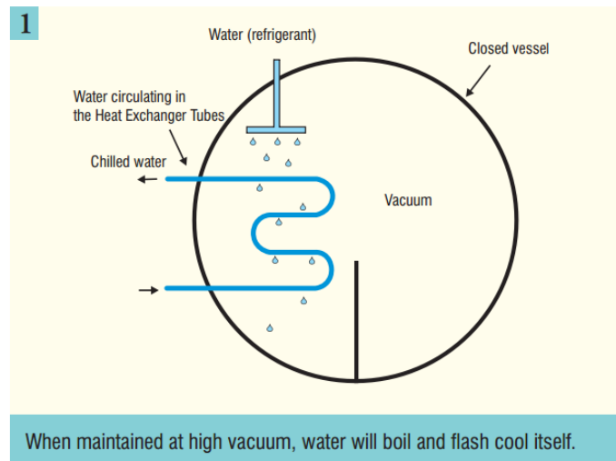
Figure 5. Trane (Thermax) Cooling System – Refrigerating Effect.
