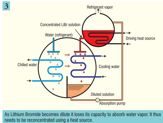
Figure 7. Trane (Thermax) Cooling System – Re-concentrated LiBr
