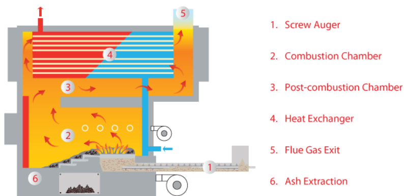
Figure 2. Stoker Boiler Diagram
